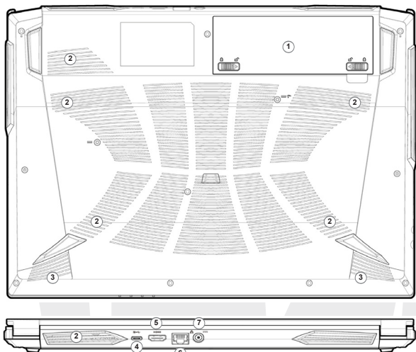
Figure 5 - Bottom & Rear Views
